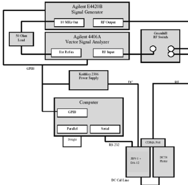
Figure 1: Tuning and alignment diagram
