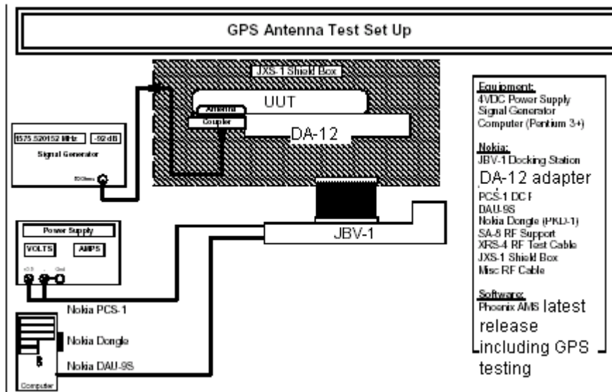
Figure 3: GPS radiated testing
