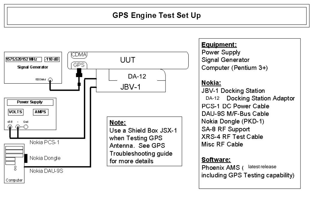
Figure 2: GPS Galvanic Testing
